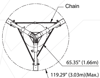
Foot Print Diameter at Maximum Height
