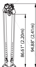
Height in Close cNdition
