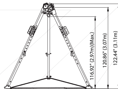
Maximum Height in Open Condition
