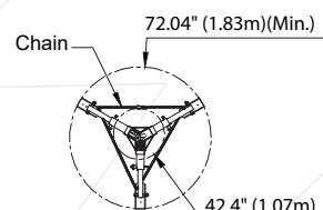
Foot Print Diameter at Minimum Height
