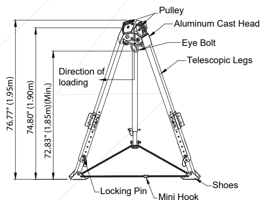
Minimum Height in Open Condition
